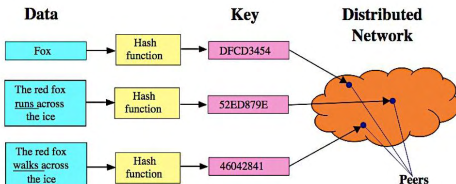
Figure 4. Distributed Hash Table
